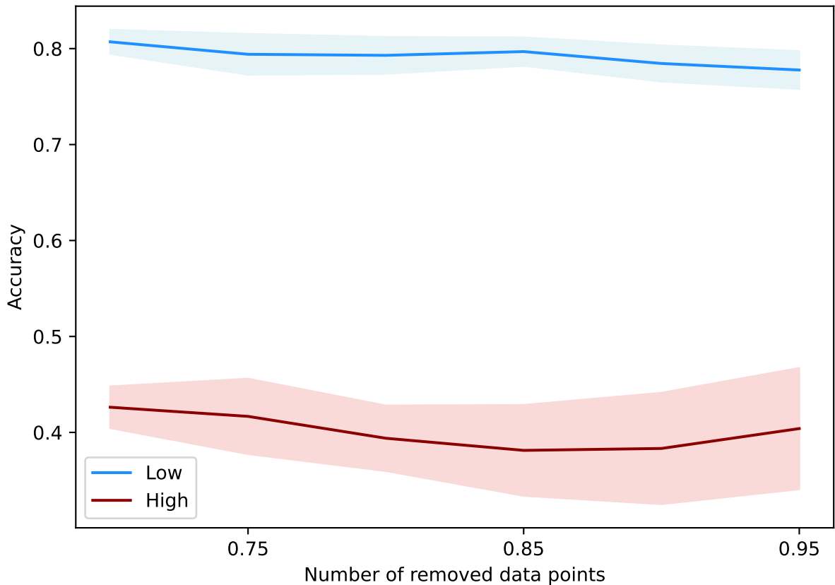
DataAttrOpt(3000, 0.03, 15, best, +b, alpha=best) - imdb-embeddings
